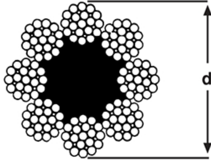
8 X 19 WARRINGTON-SEALE 8 [ 1 + 6 + ( 6 + 6 ) ]
