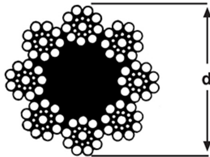
8 X 19 SEALE 8 (1 + 9 + 9)
