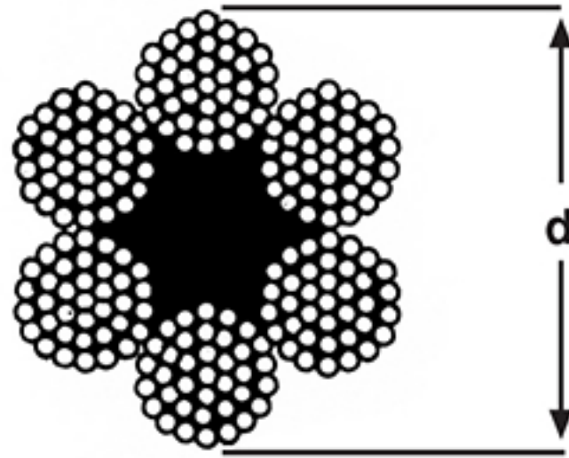
6 X 37 STANDARD 6 (1 + 6 + 12 + 8)
